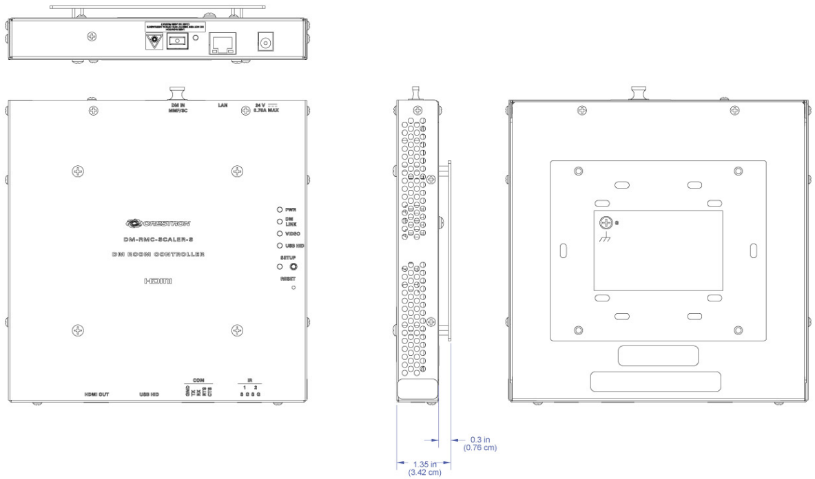
UNIT WITH BRACKET INSTALLED
